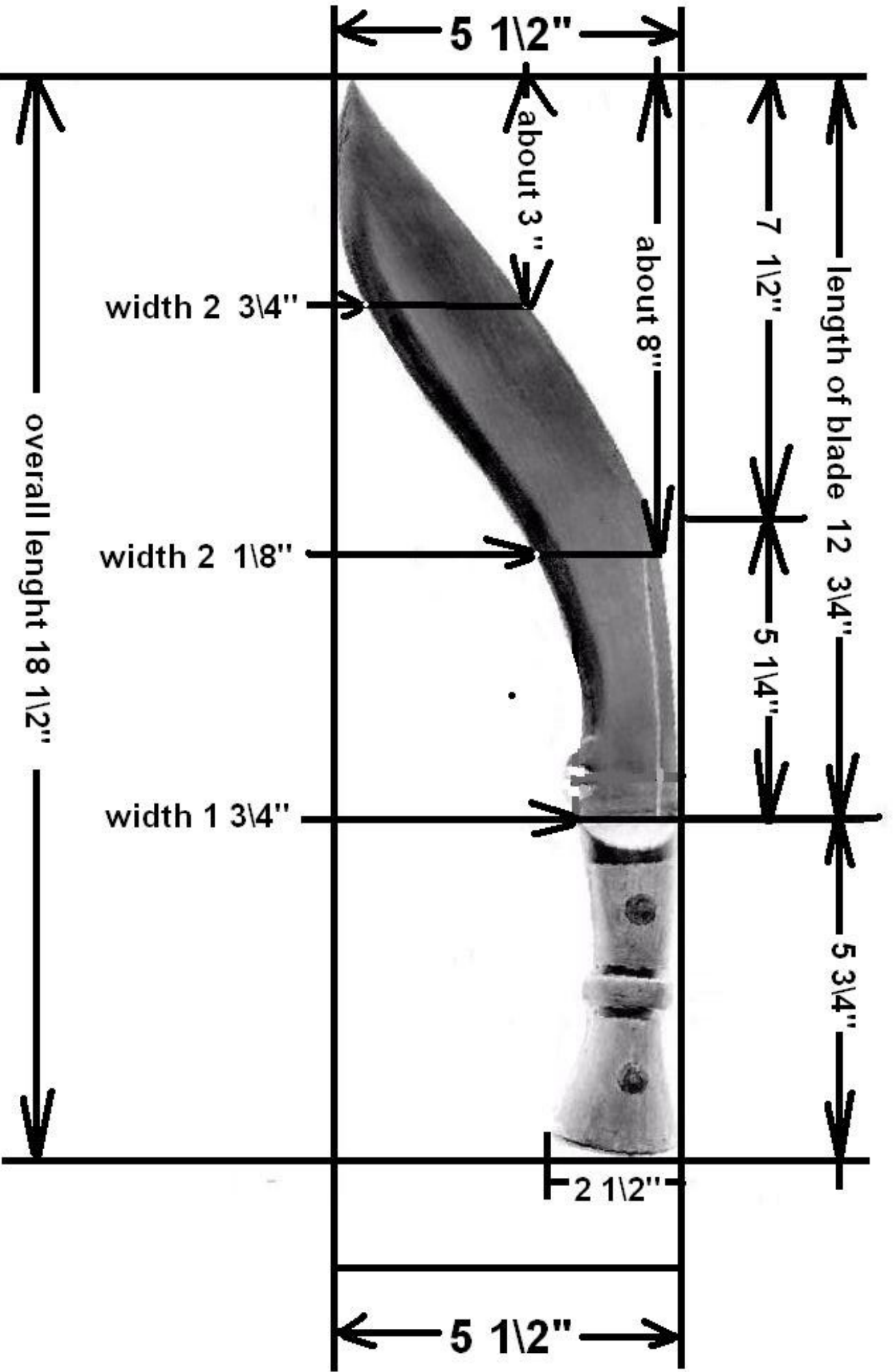
Dimension Sketch 1 K45 Kukri
